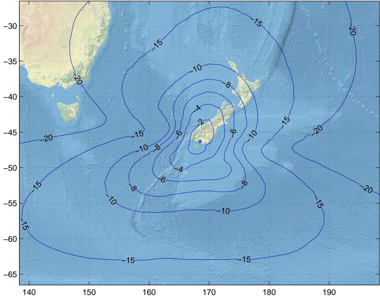
Gain Contours at 550km for IVC. Beam ID=SRX, Polarization=lhcp
