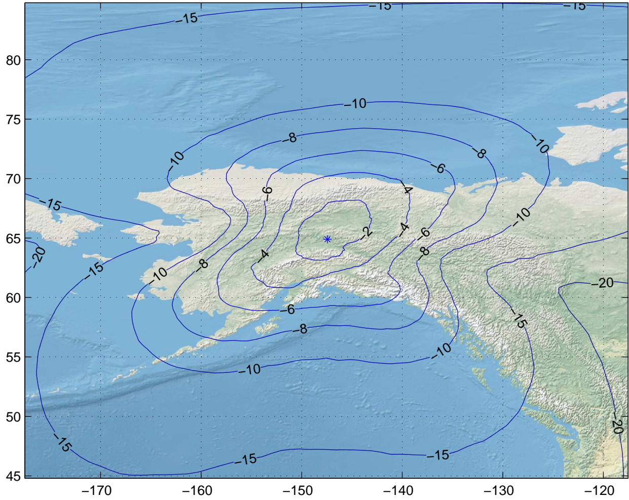
Gain Contours at 585km for FAI. Beam ID=SRX, Polarization=lhcp
