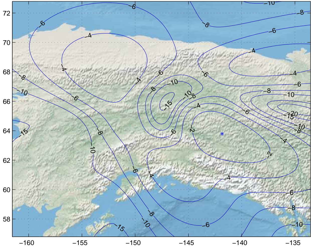
Gain Contours at 460km for FAI. Beam ID=URC, Polarization=h
