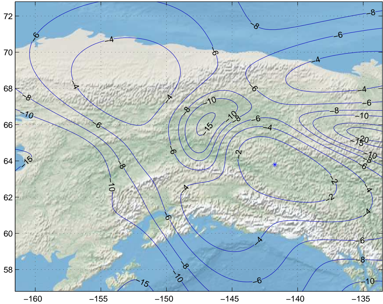
Gain Contours at 475km for FAI. Beam ID=URC, Polarization=h
