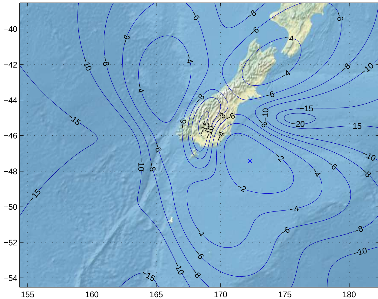
Gain Contours at 475km for IVC. Beam ID=URC, Polarization=h
