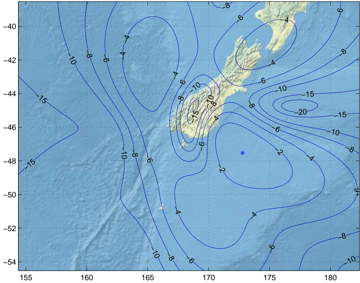
Gain Contours at 550km for IVC. Beam ID=URC, Polarization=h
