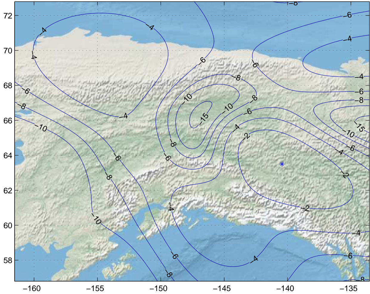
Gain Contours at 585km for FAI. Beam ID=URC, Polarization=h
