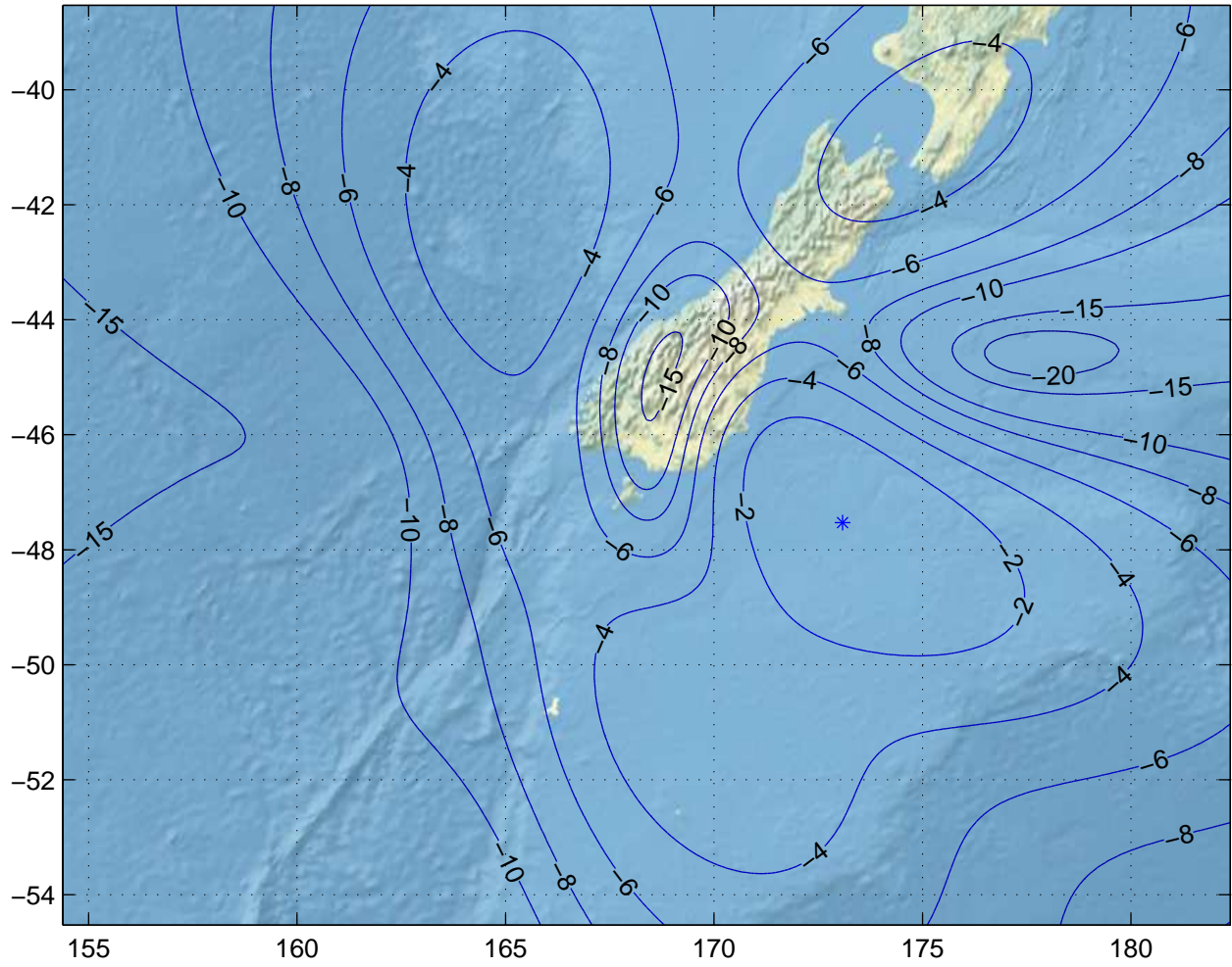
Gain Contours at 585km for IVC. Beam ID=URC, Polarization=h
