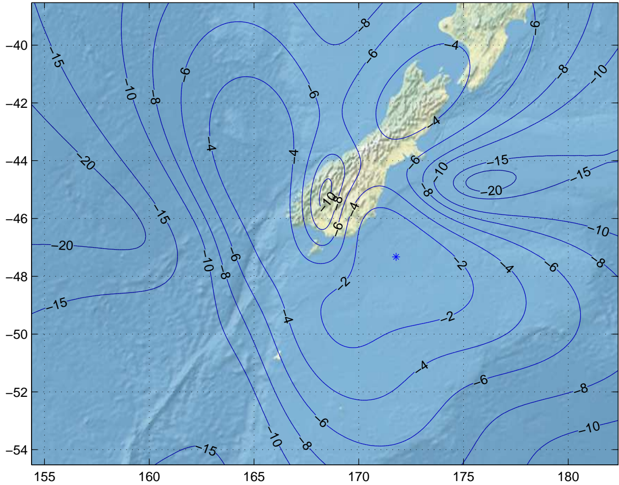
Gain Contours at 460km for IVC. Beam ID=UTC, Polarization=h
