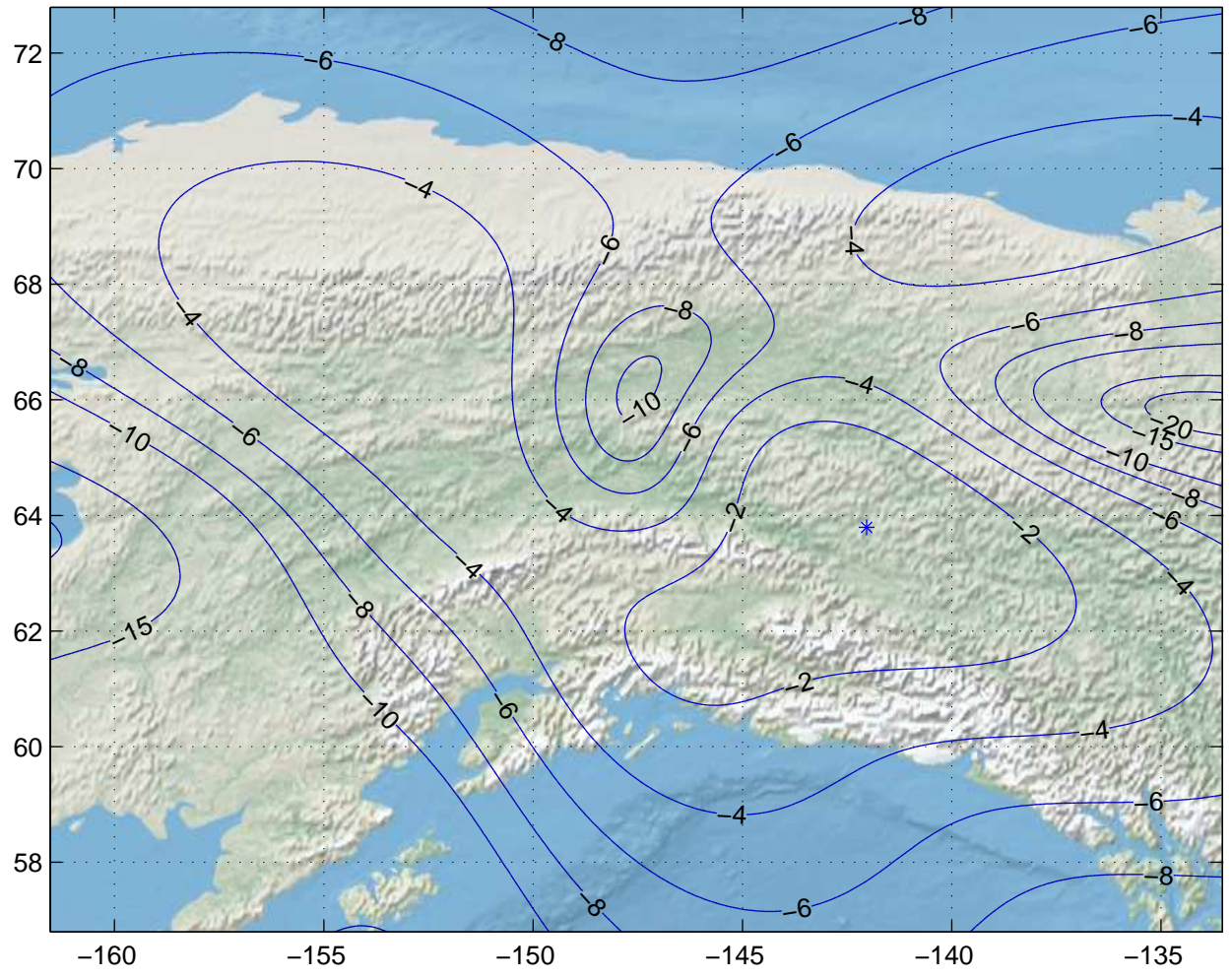
Gain Contours at 475km for FAI. Beam ID=UTC, Polarization=h
