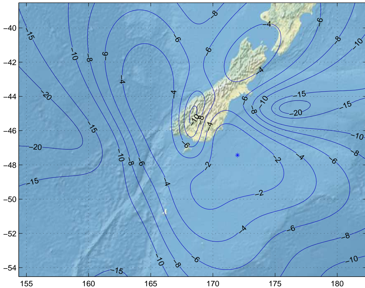
Gain Contours at 475km for IVC. Beam ID=UTC, Polarization=h
