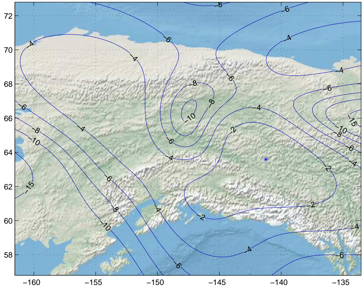
Gain Contours at 550km for FAI. Beam ID=UTC, Polarization=h
