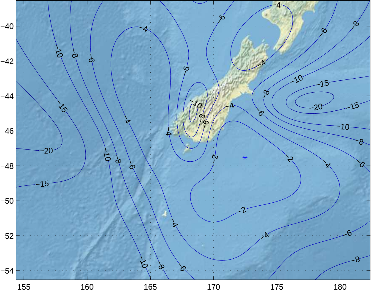
Gain Contours at 550km for IVC. Beam ID=UTC, Polarization=h
