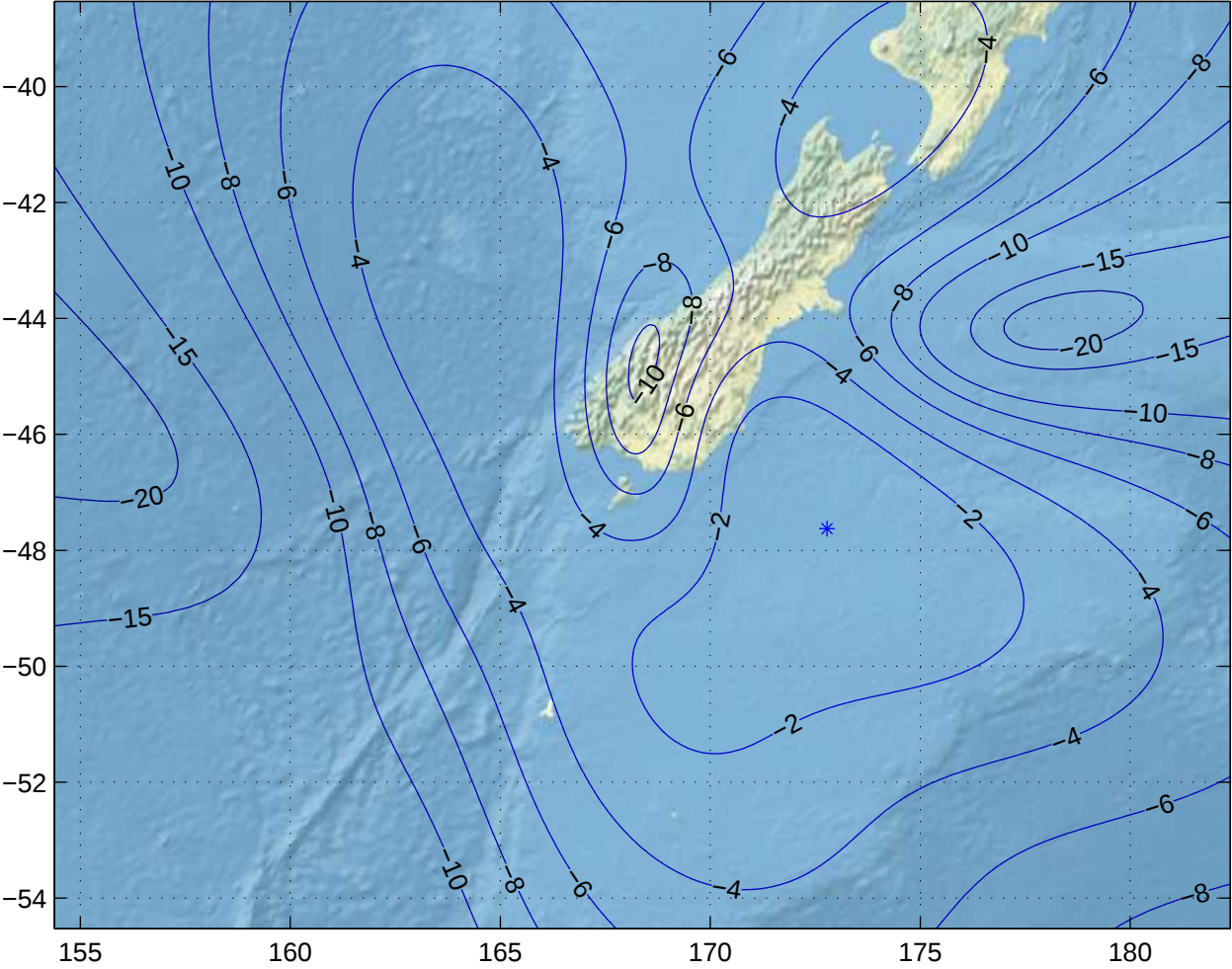
Gain Contours at 585km for IVC. Beam ID=UTC, Polarization=h
