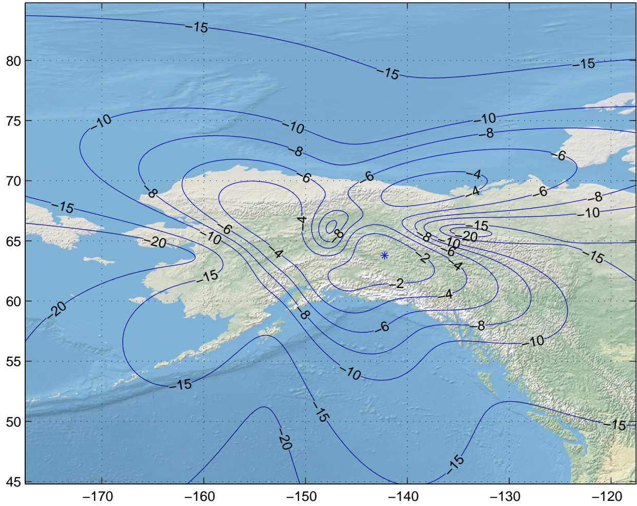
Gain Contours at 460km for FAI. Beam ID=UTX, Polarization=rhcp
