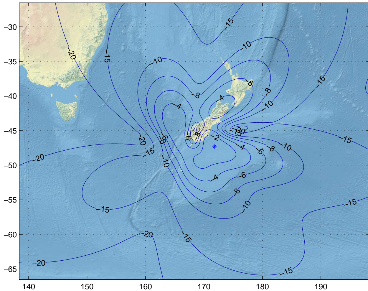
Gain Contours at 460km for IVC. Beam ID=UTX, Polarization=rhcp
