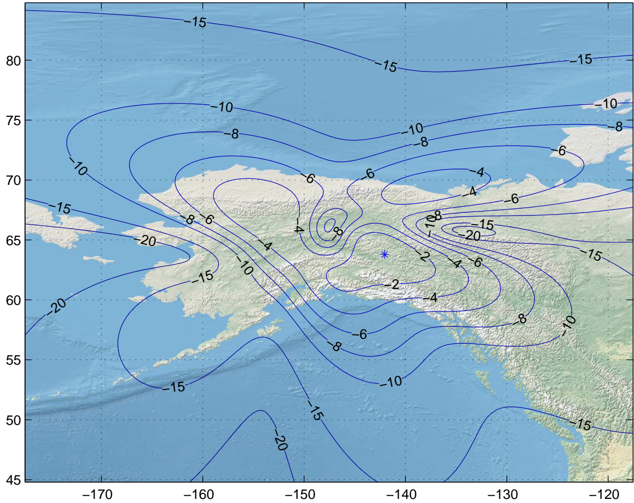
Gain Contours at 475km for FAI. Beam ID=UTX, Polarization=rhcp
