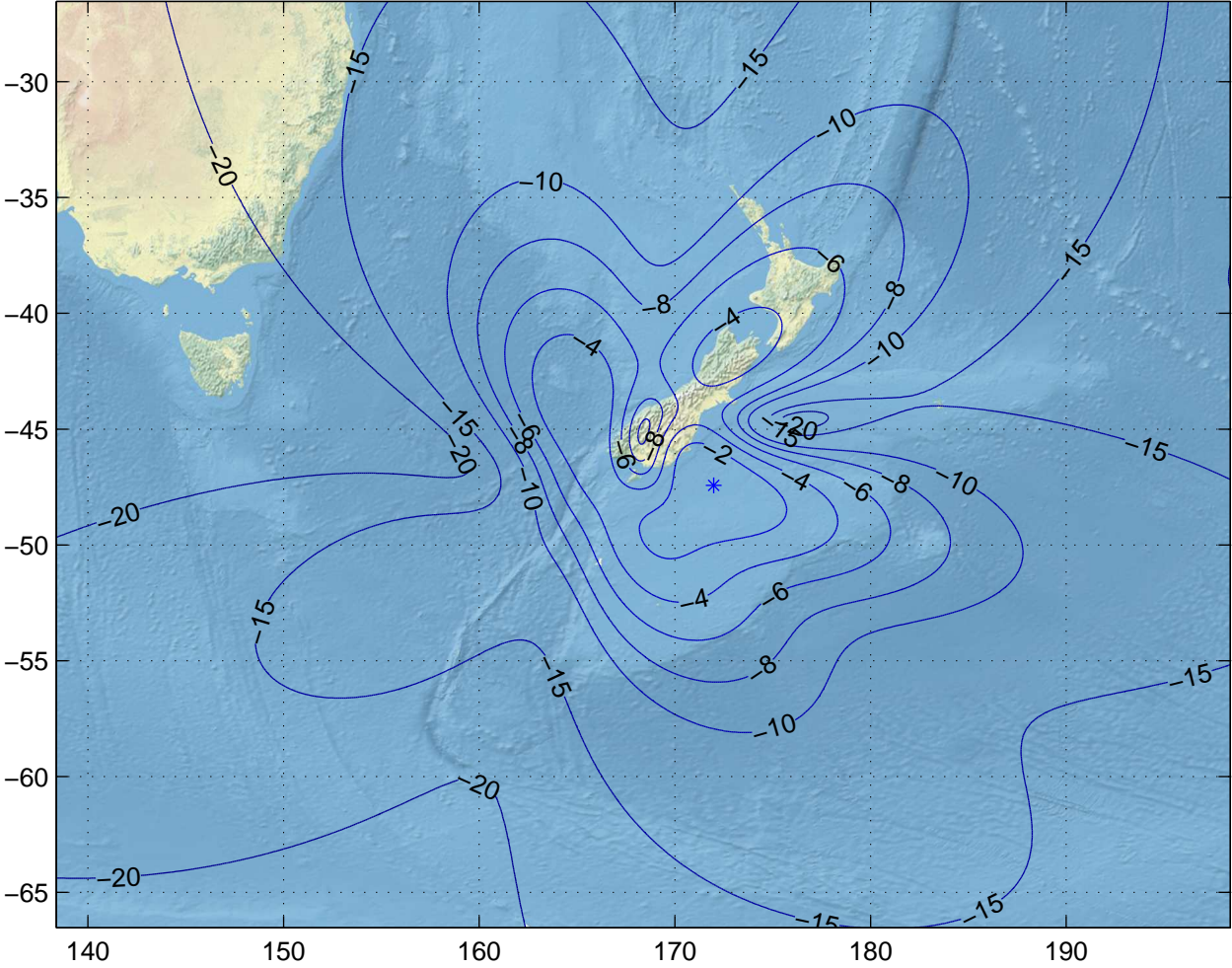
Gain Contours at 475km for IVC. Beam ID=UTX, Polarization=rhcp
