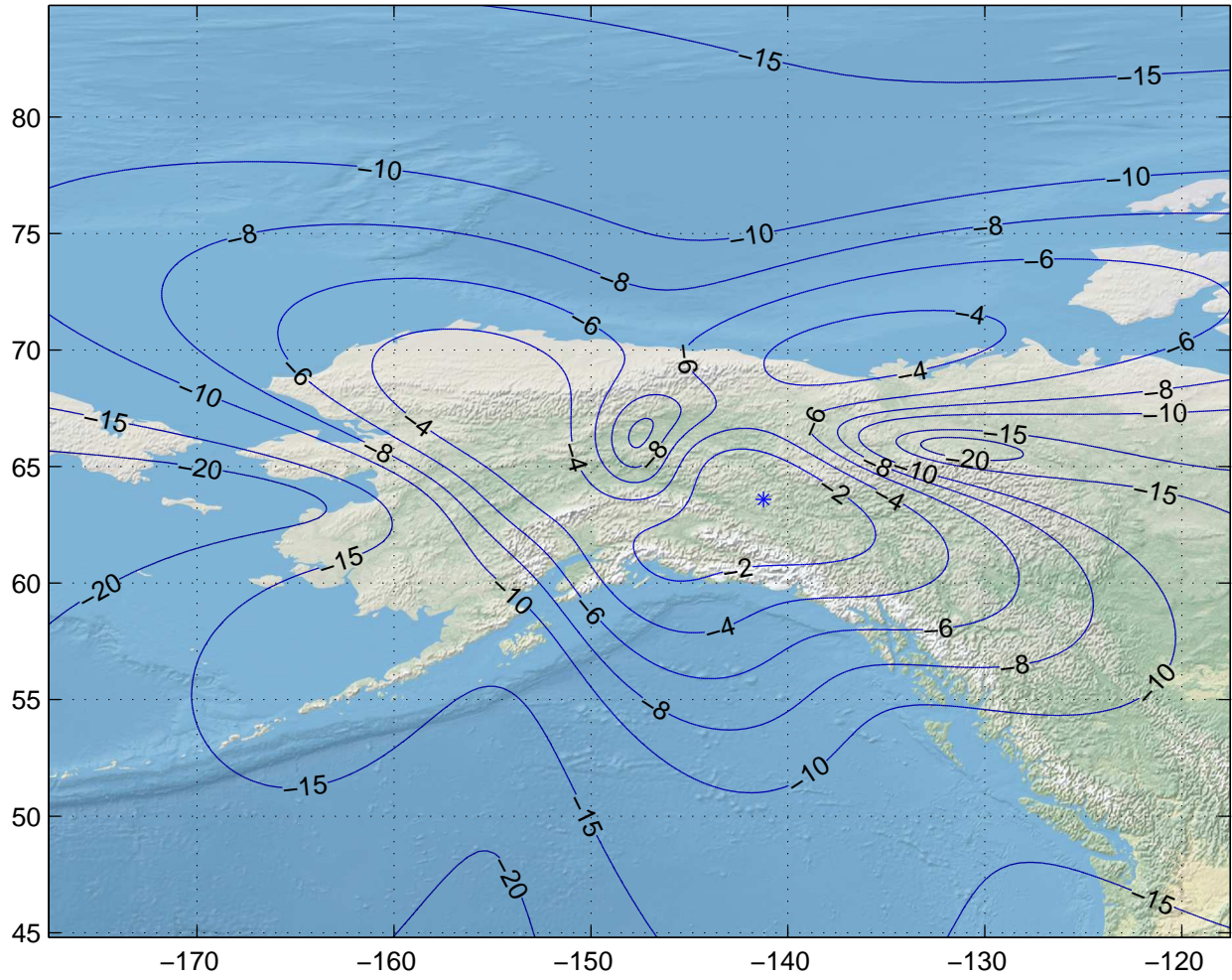
Gain Contours at 550km for FAI. Beam ID=UTX, Polarization=rhcp
