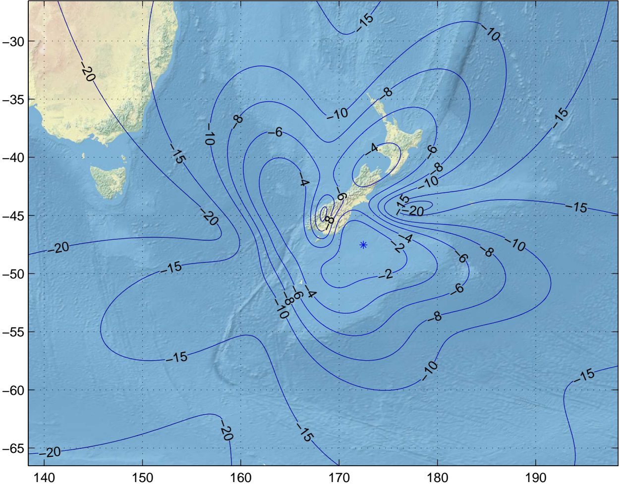
Gain Contours at 550km for IVC. Beam ID=UTX, Polarization=rhcp
