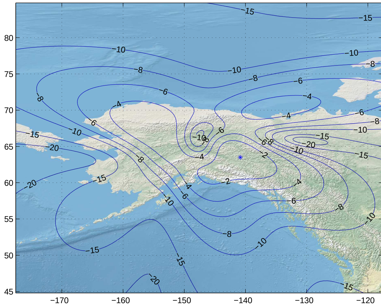
Gain Contours at 585km for FAI. Beam ID=UTX, Polarization=rhcp
