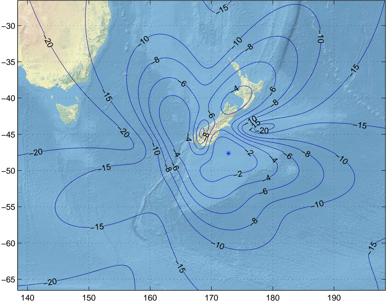
Gain Contours at 585km for IVC. Beam ID=UTX, Polarization=rhcp
