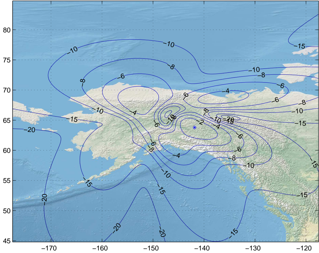
Gain Contours at 460km for FAI. Beam ID=URX, Polarization=rhcp
