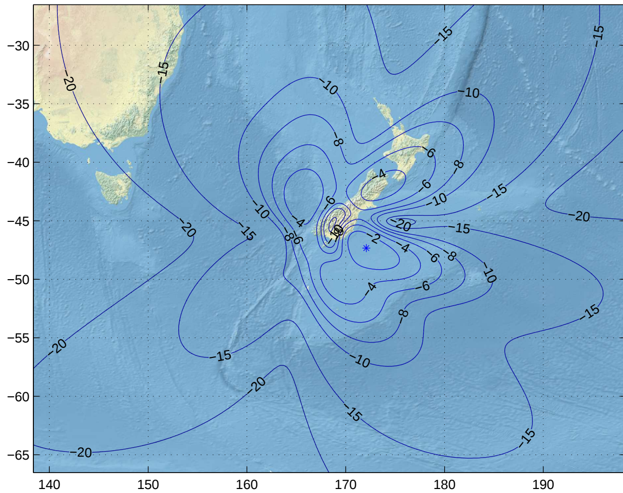
Gain Contours at 460km for IVC. Beam ID=URX, Polarization=rhcp
