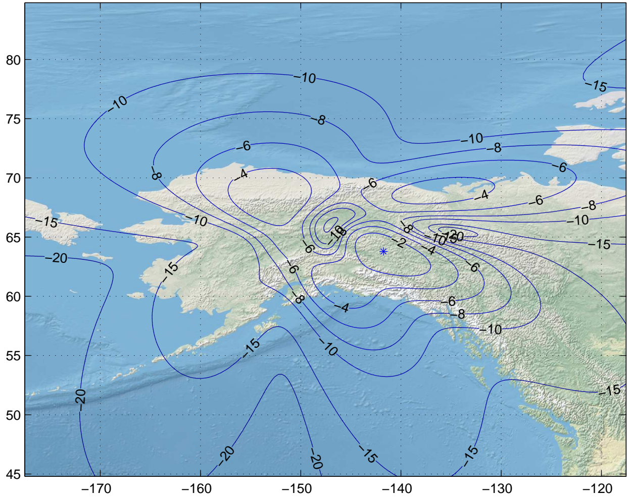
Gain Contours at 475km for FAI. Beam ID=URX, Polarization=rhcp
