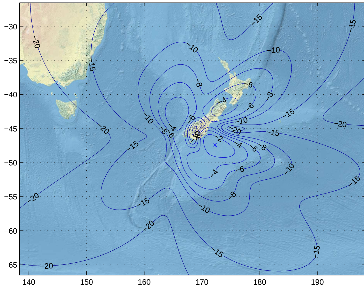
Gain Contours at 475km for IVC. Beam ID=URX, Polarization=rhcp
