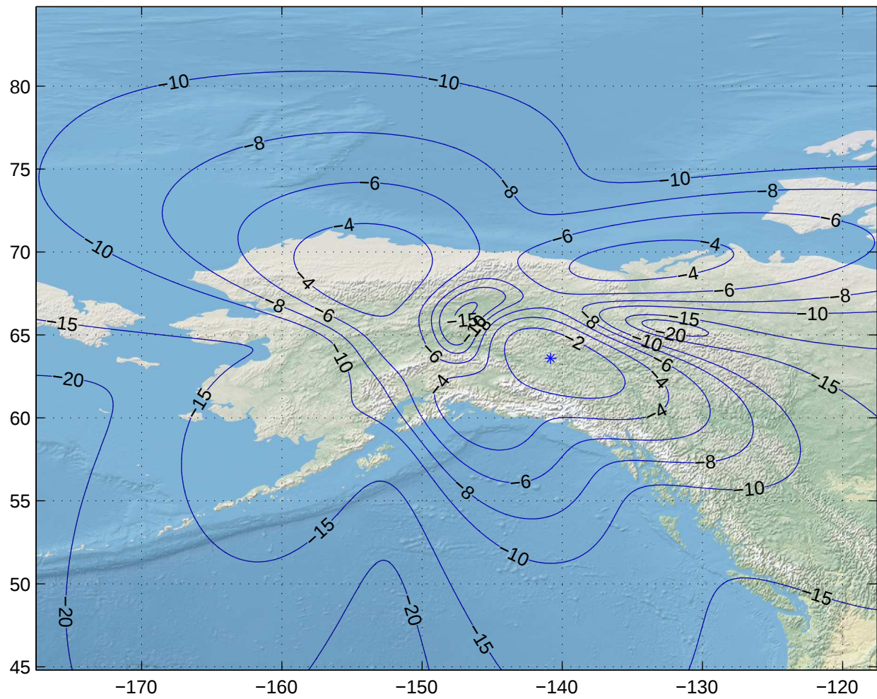
Gain Contours at 550km for FAI. Beam ID=URX, Polarization=rhcp
