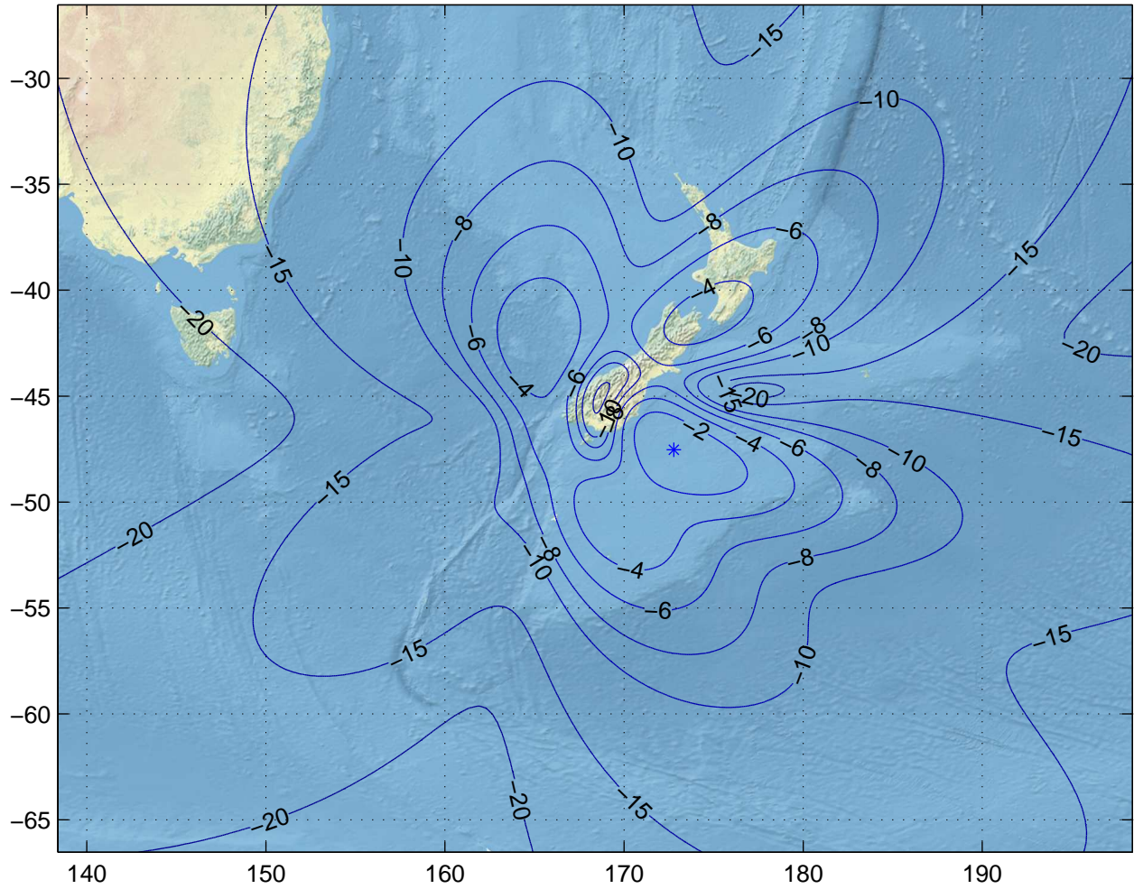
Gain Contours at 550km for IVC. Beam ID=URX, Polarization=rhcp
