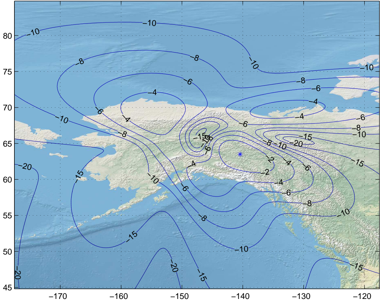
Gain Contours at 585km for FAI. Beam ID=URX, Polarization=rhcp
