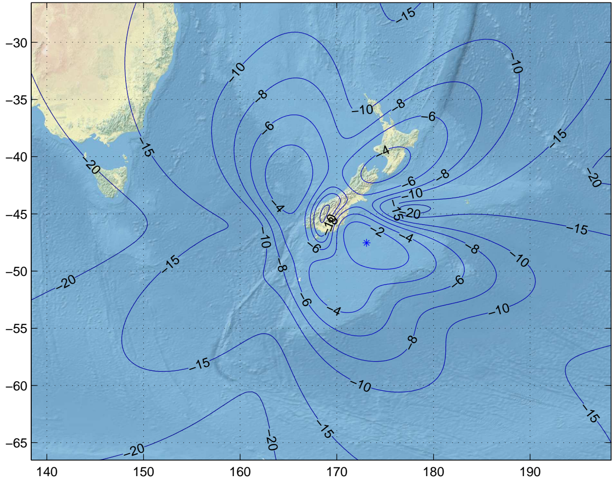
Gain Contours at 585km for IVC. Beam ID=URX, Polarization=rhcp
