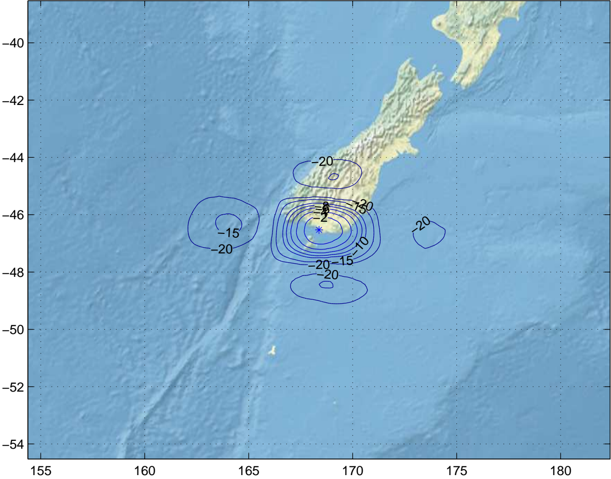
Gain Contours at 460km for IVC. Beam ID=XTC, Polarization=rhcp
