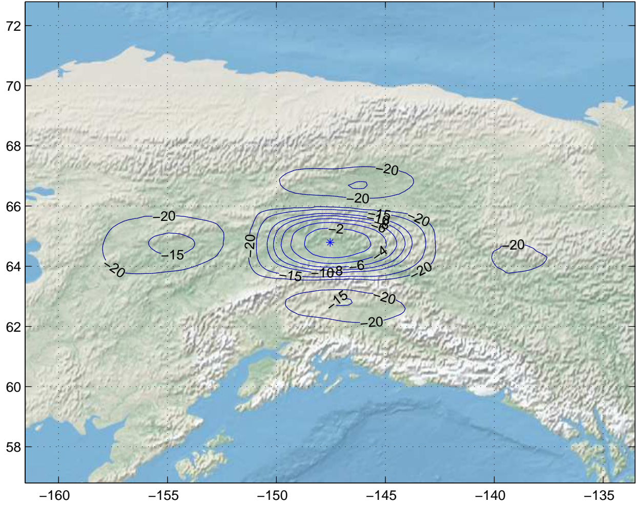
Gain Contours at 475km for FAI. Beam ID=XTC, Polarization=rhcp
