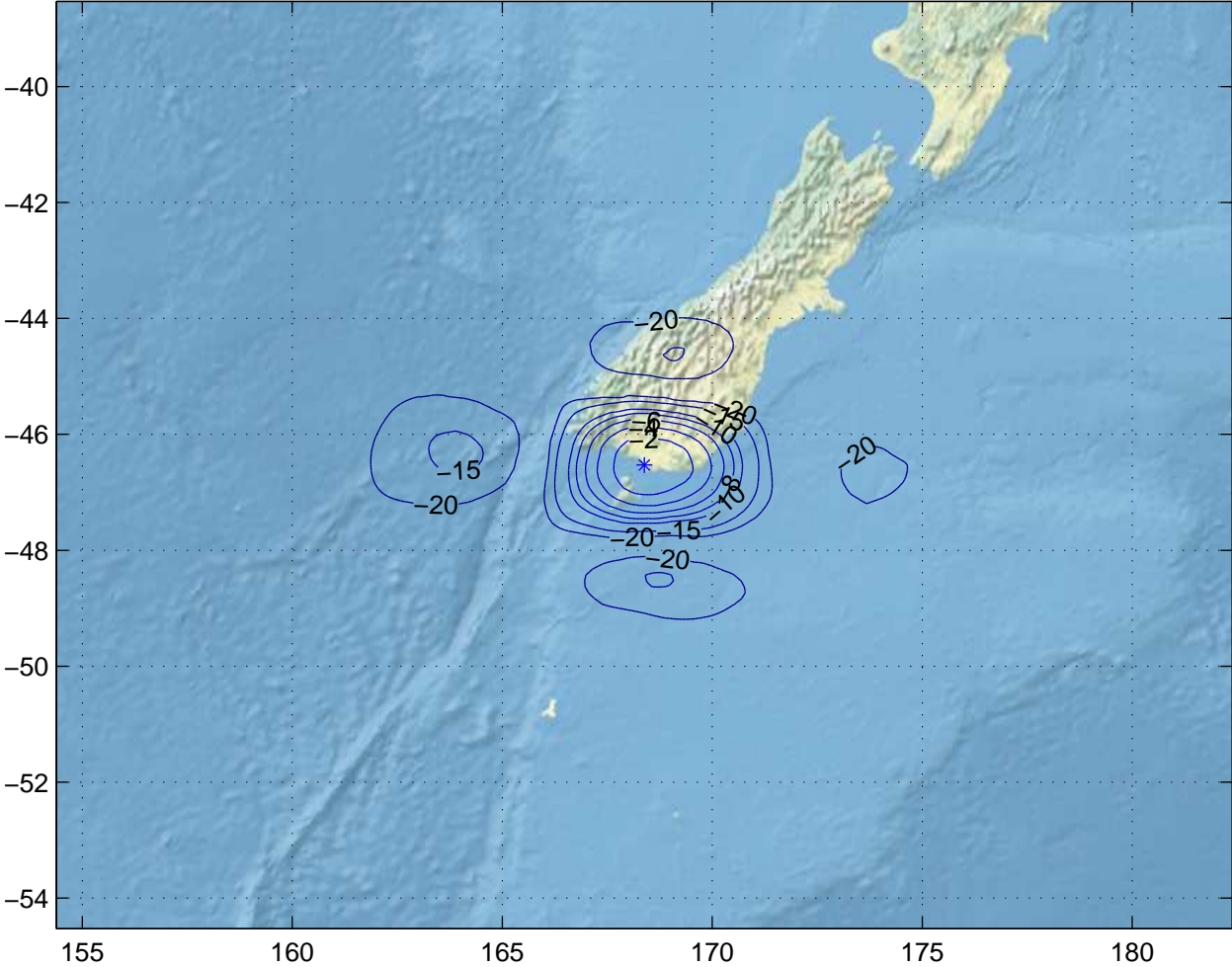
Gain Contours at 475km for IVC. Beam ID=XTC, Polarization=rhcp
