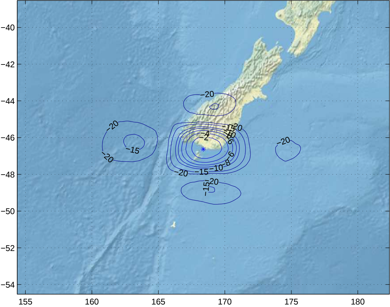
Gain Contours at 550km for IVC. Beam ID=XTC, Polarization=rhcp
