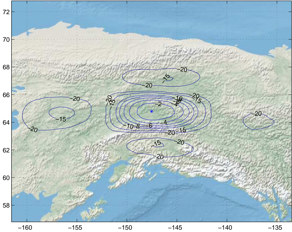
Gain Contours at 585km for FAI. Beam ID=XTC, Polarization=rhcp
