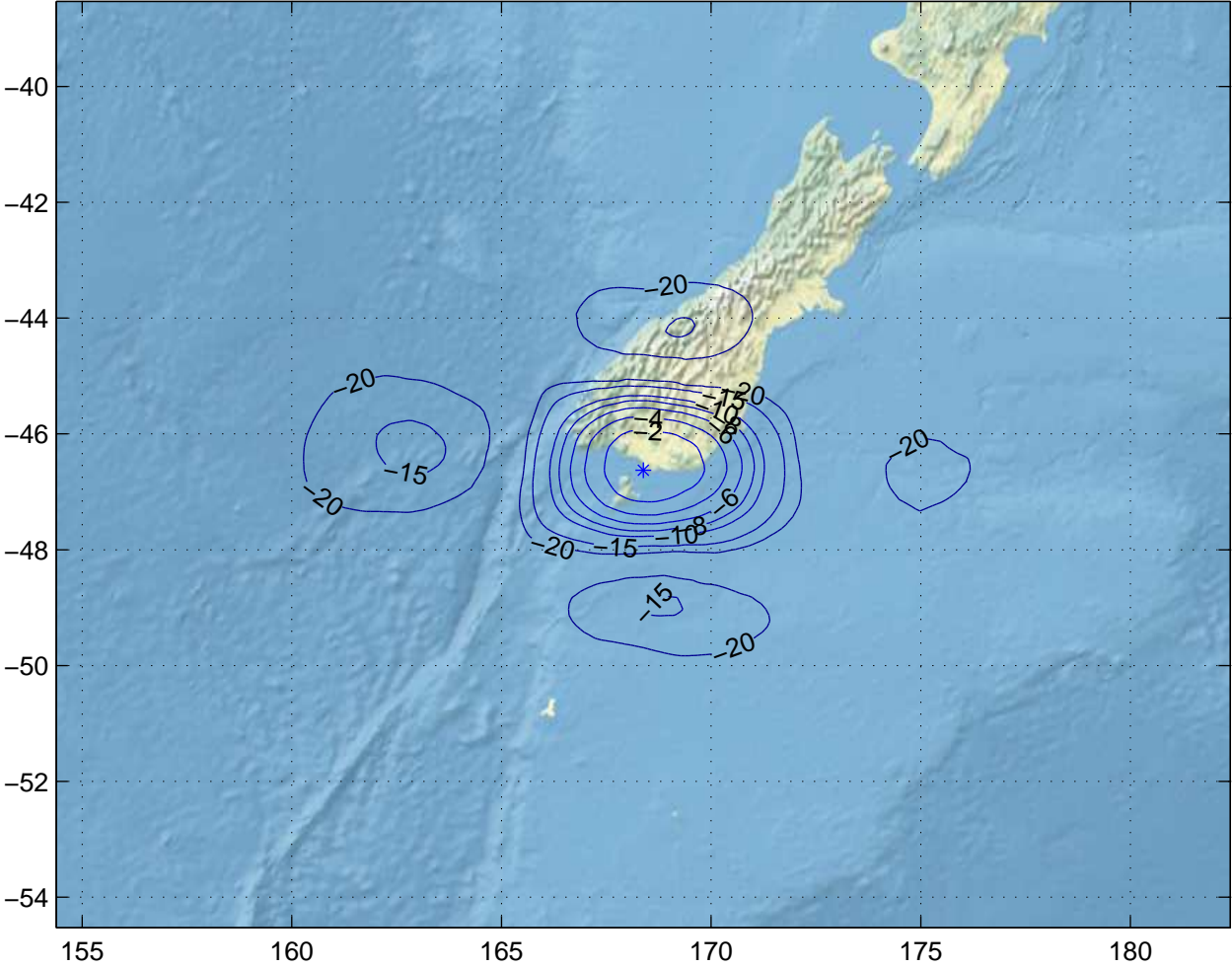
Gain Contours at 585km for IVC. Beam ID=XTC, Polarization=rhcp
