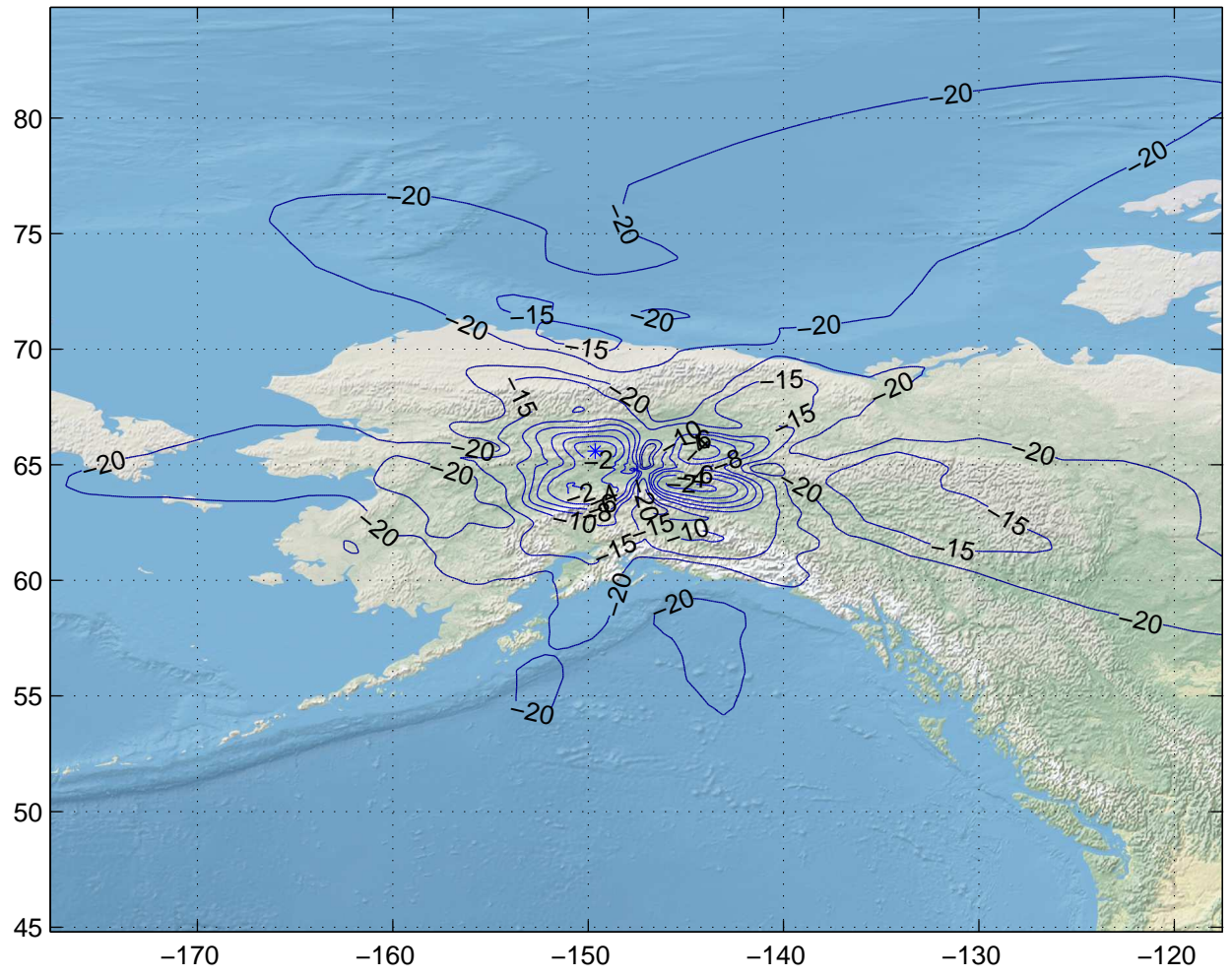
Gain Contours at 460km for FAI. Beam ID=XTX, Polarization=lhcp
