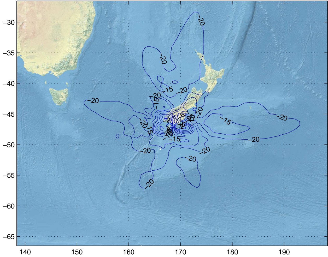
Gain Contours at 460km for IVC. Beam ID=XTX, Polarization=lhcp
