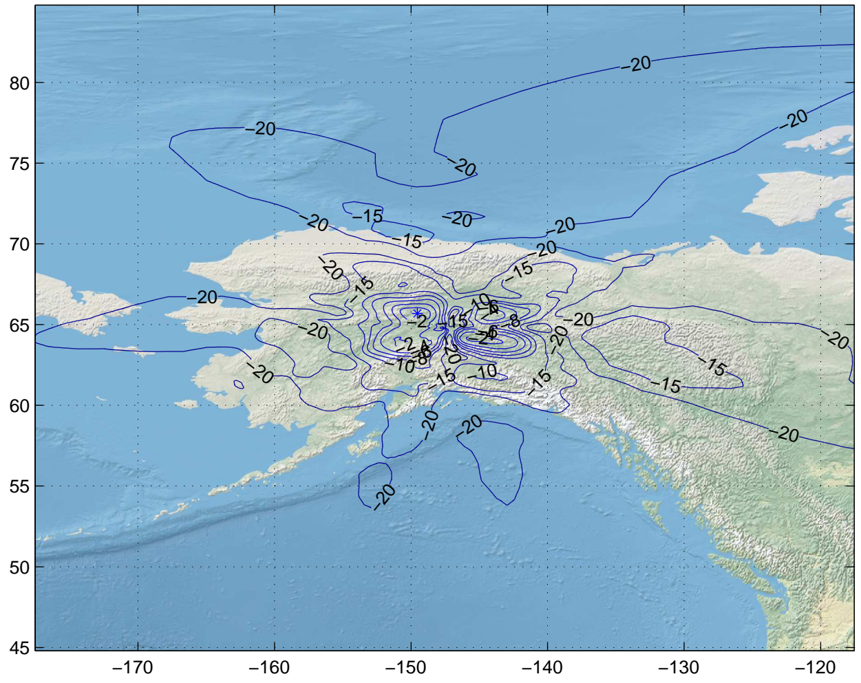
Gain Contours at 475km for FAI. Beam ID=XTX, Polarization=lhcp
