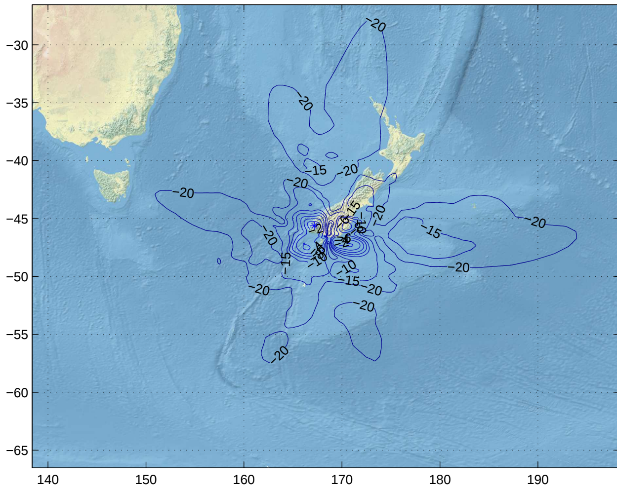
Gain Contours at 475km for IVC. Beam ID=XTX, Polarization=lhcp
