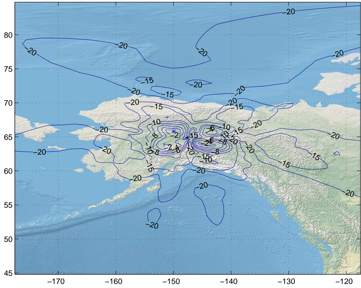
Gain Contours at 550km for FAI. Beam ID=XTX, Polarization=lhcp
