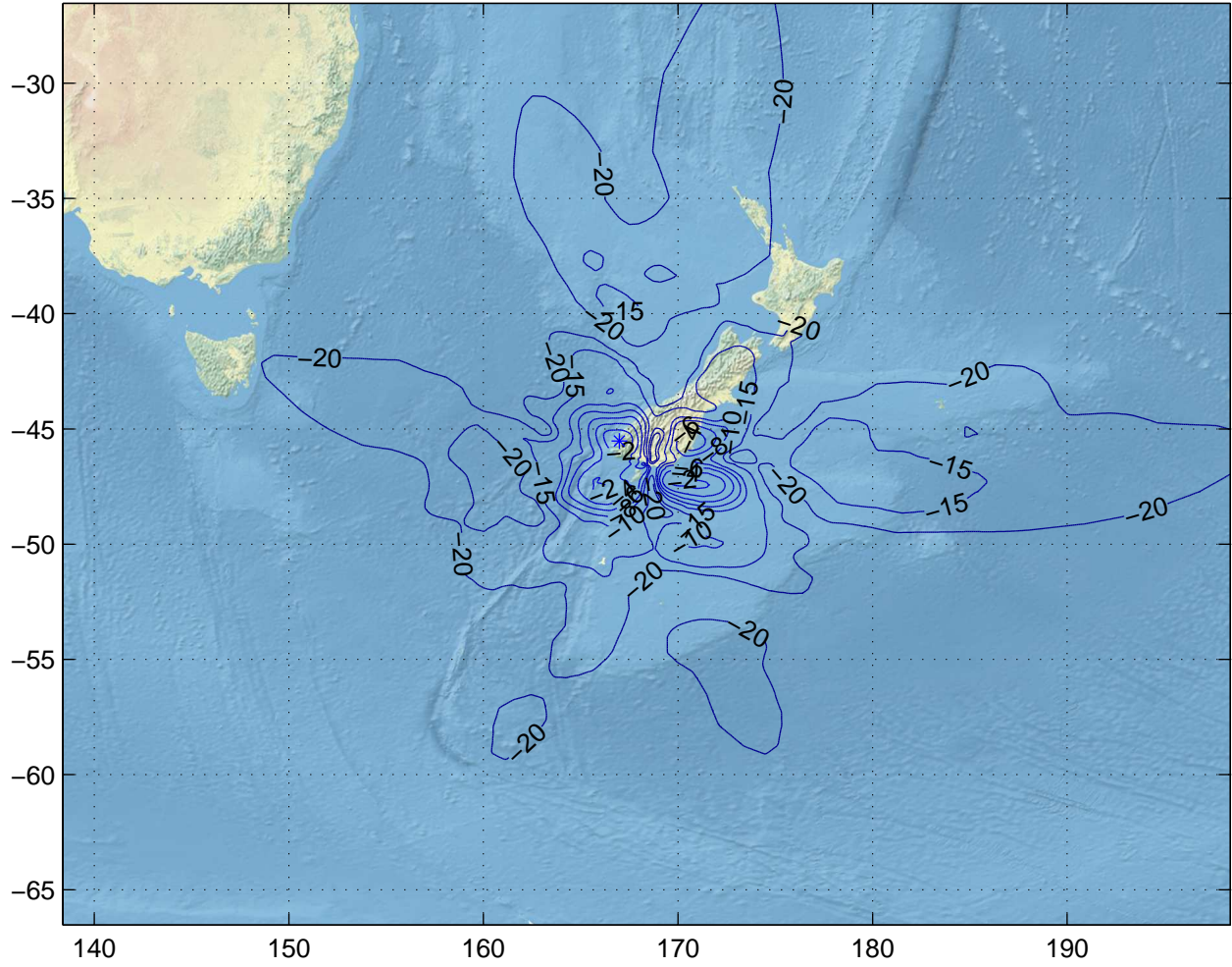
Gain Contours at 550km for IVC. Beam ID=XTX, Polarization=lhcp
