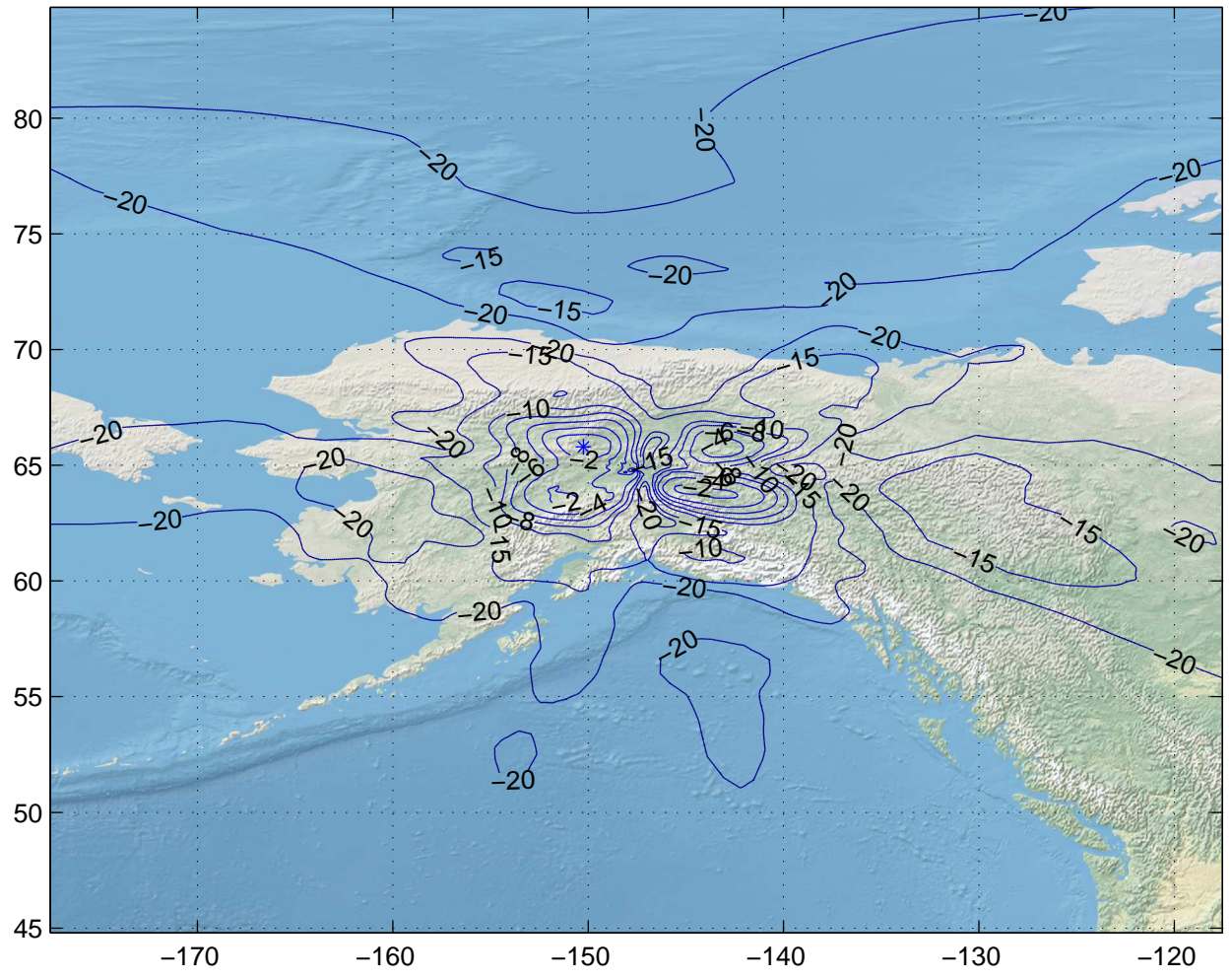
Gain Contours at 585km for FAI. Beam ID=XTX, Polarization=lhcp
