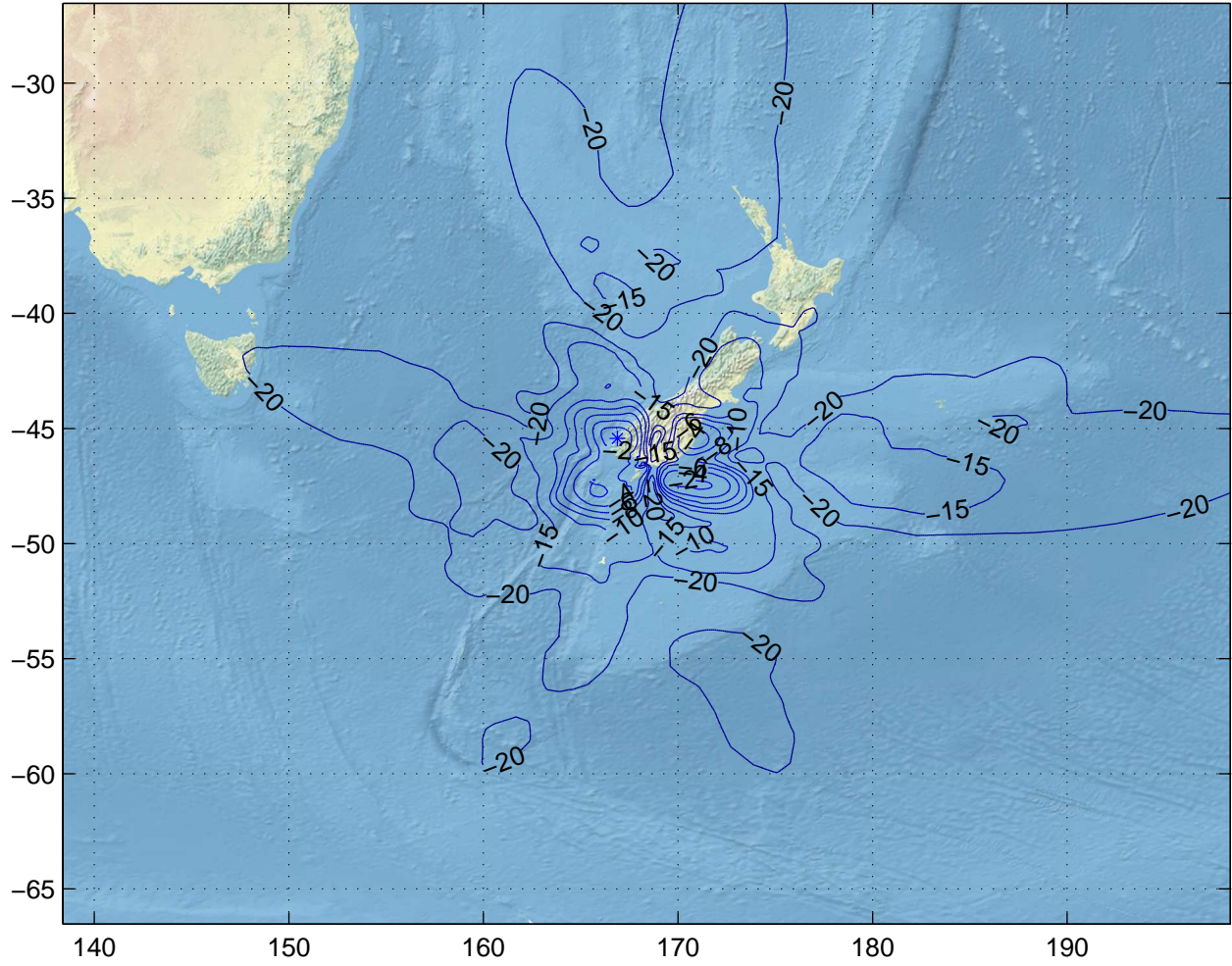
Gain Contours at 585km for IVC. Beam ID=XTX, Polarization=lhcp
