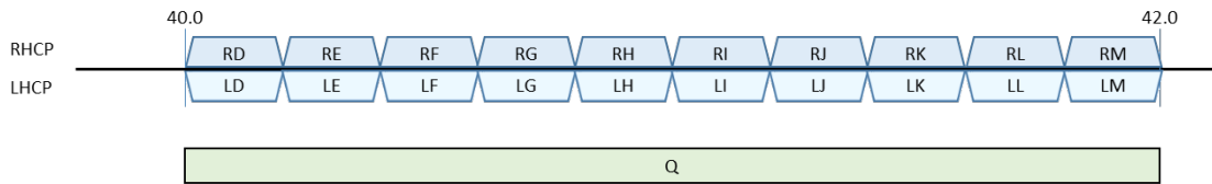
Figure 4-2. Frequency plan for the return link
