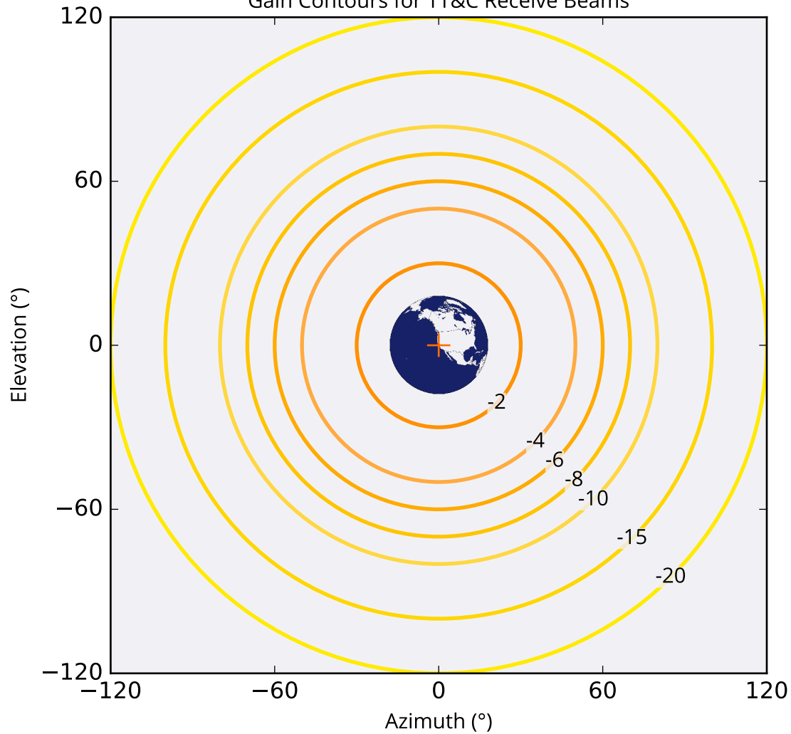
Gain Contours for TT&C Receive Beams
