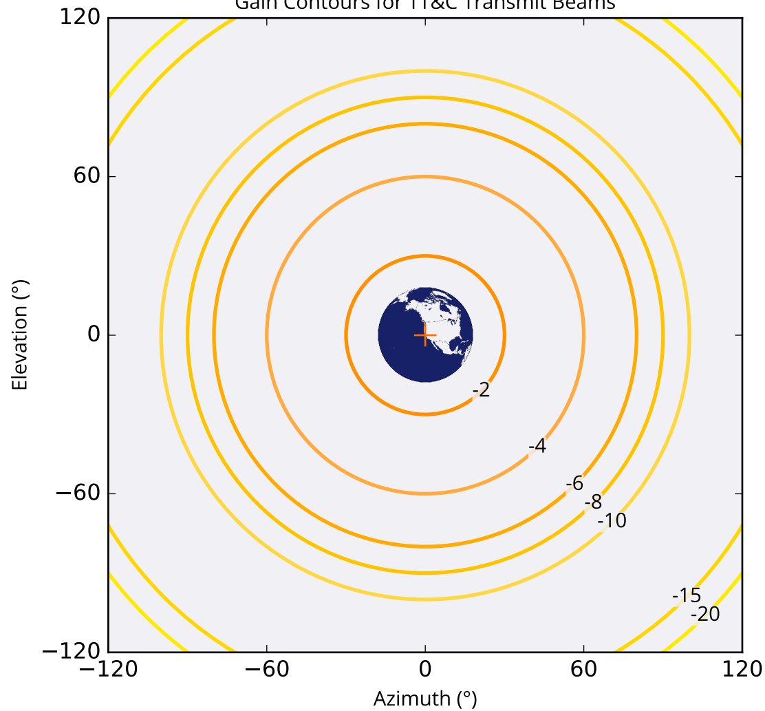
Gain Contours for TT&C Transmit Beams
