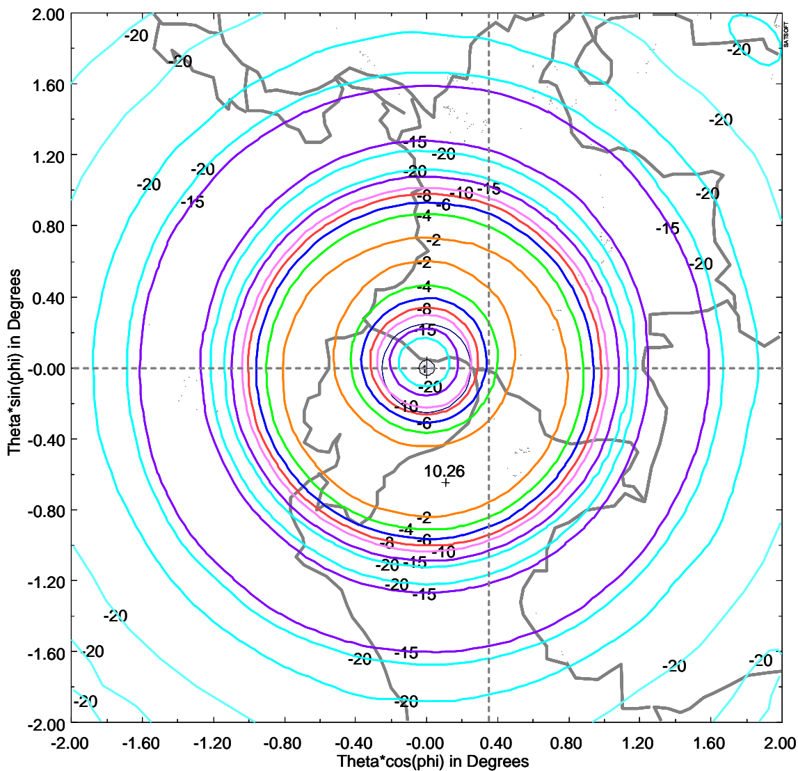
GSO Satellite at 77W Receive Antenna Contours – XPol (Contour Levels: -2, -4, -6, -8, -10, -15, -20 dB)
