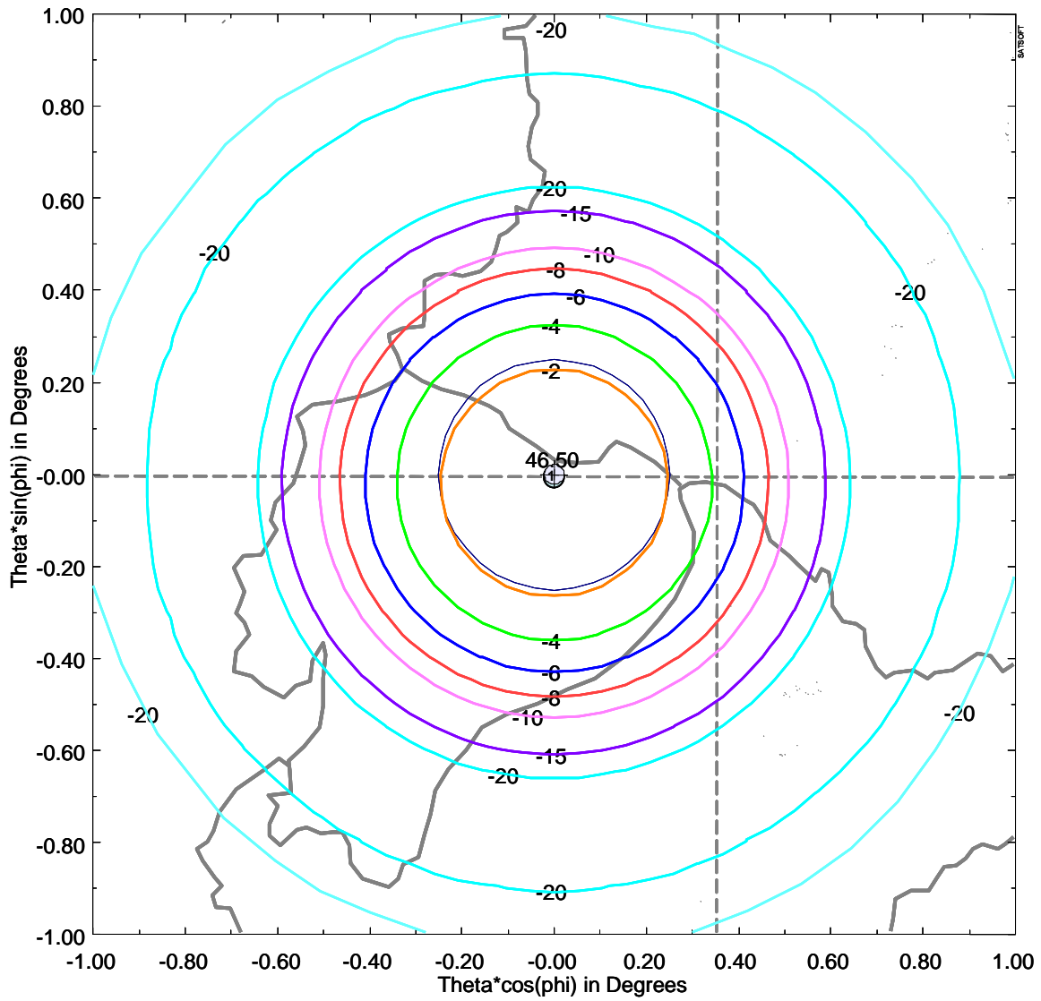
GSO Satellite at 77W Receive Antenna Contours – CoPol (Contour Levels: -2, -4, -6, -8, -10, -15, - 20 dB)
