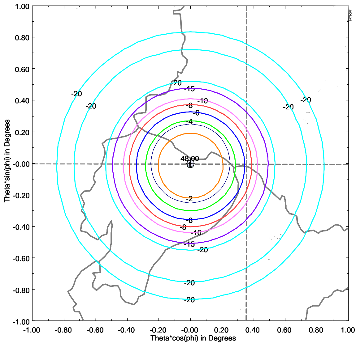
GSO Satellite at 77W Transmit Antenna Contours – CoPol (Contour Levels: -2, -4, -6, -8, -10, -15, - 20 dB)
